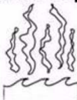
Water Vapor
