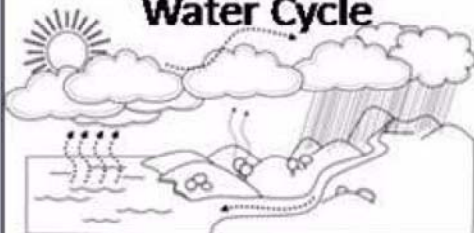
Water Cycle
